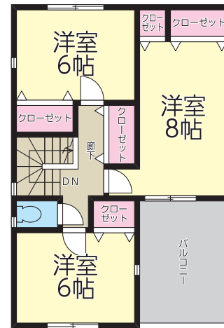
2F:56.70㎡
