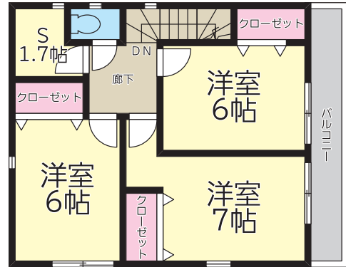
2F:45.36㎡
